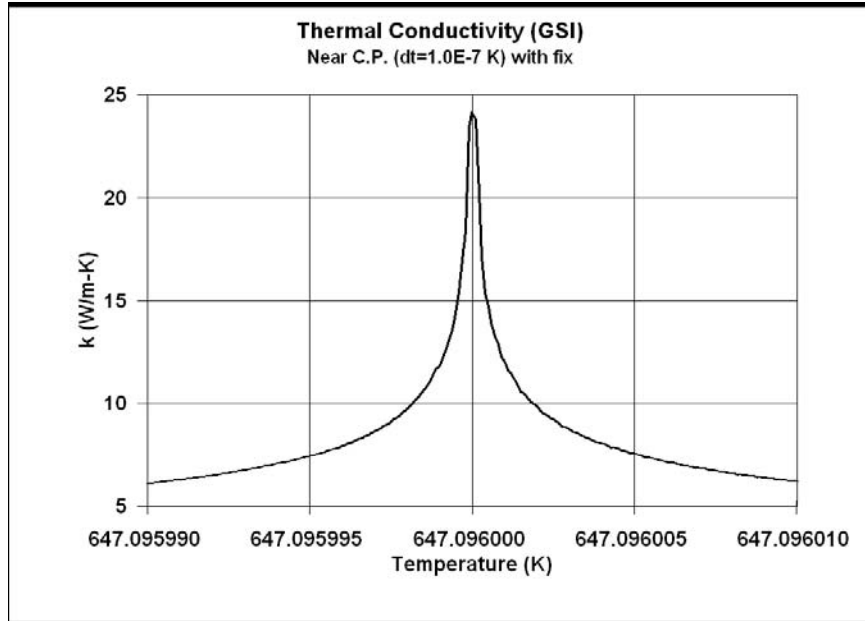
Figure 5 - k_{\text{GSI}} near critical point, \Delta T=1.0 \times 10^{-7} K with fix
