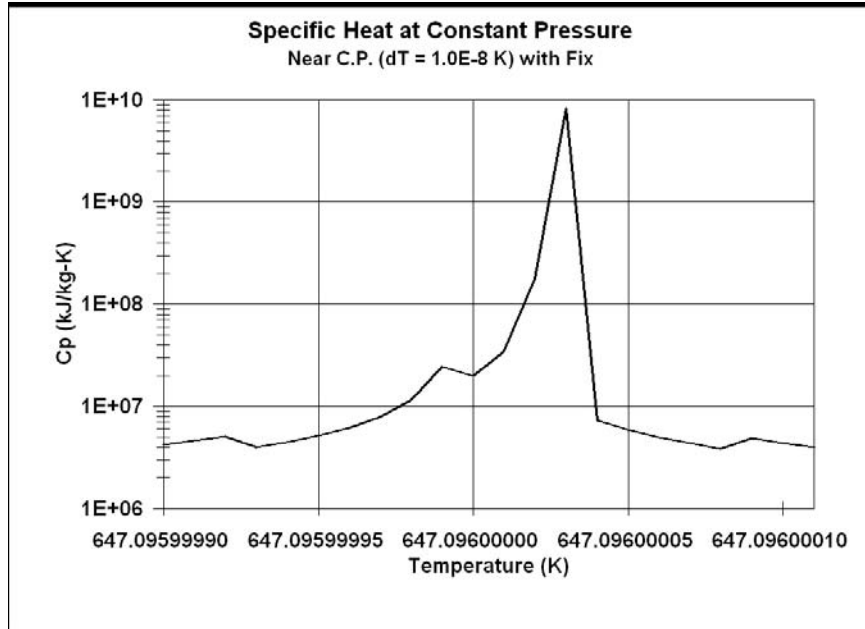
Figure 2 - C_p near critical point, \Delta T=1.0 \times 10^{-8} K with fix
