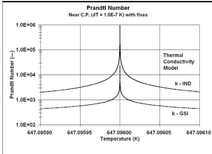
Figure 7 - Prandtl number (Pr) based on k_{GSI} and k_{IND}
