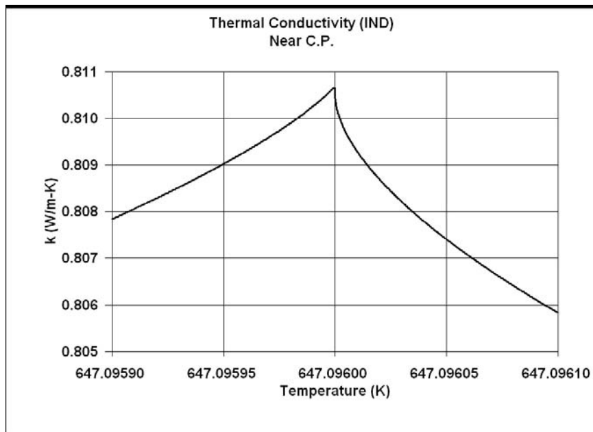
Figure 6 - k_{\text{IND}} near critical point, \Delta T=1.0 \times 10^{-7} K
