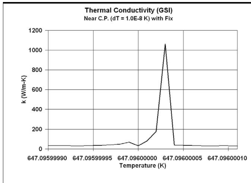
Figure 4 - k_{GSI} near critical point, \Delta T = 1.0 \times 10^{-8} K with fix
