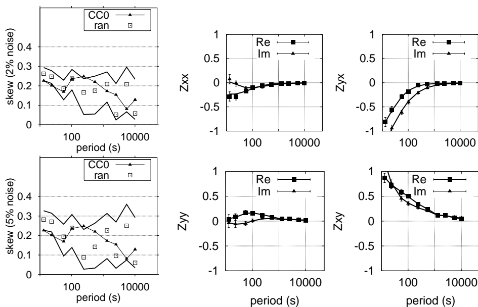
Fig. 4. An example of skew values using synthetic data (left), estimated from the tensor elements shown in right (units in km/s). The elements of the model response (lines) are shown over the data scattered with 5% Gaussian noise (dots). The skew of the model response (CC0; in Fig. 3) is shown over the noisy skew (ran) within its 95% confidence limit. Above: Skew from the elements with 2% Gaussian noise. Below: Skew from the elements with 5% Gaussian noise.
