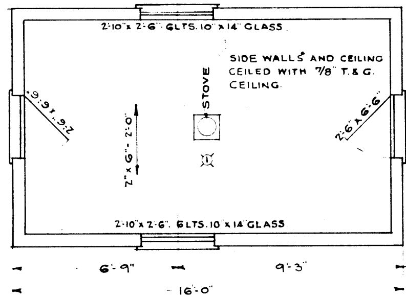
FIRST FLOOR PLAN Scale: 1/4" = 1'-0"
